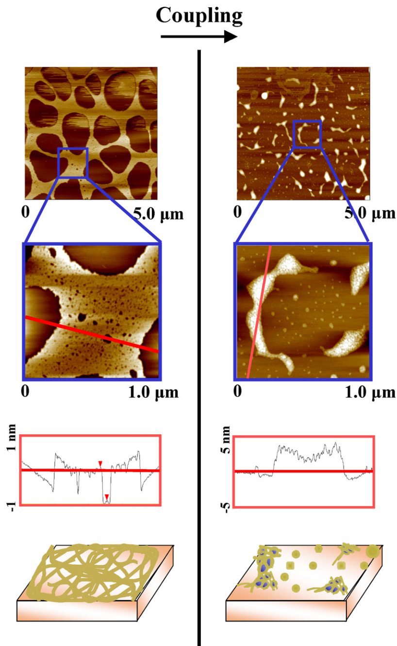
Fig. 8. AFM images, section analyses, and schematic illustration of NaPGA and its coupling-reacted composite with dendrimer at [1/0.01]. NaPGA concentration = 0.04 wt%.
