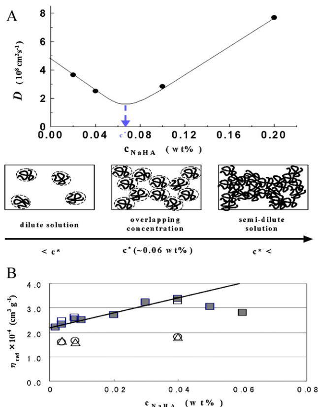
Fig. 2. (A) Apparent diffusion coefficients D of aqueous NaHA solutions as a function of NaHA concentration c_{\text{NaHA}} . c^* is an overlap threshold concentration. (B) Reduced viscosities \eta_{\text{red}} of aqueous NaHA solutions with and without coupling reaction with dendrimers as a function of NaHA concentration c_{\text{NaHA}} . [NaHA residue/dendrimer]: closed square, [1/0]; open square, [1/0.001] with coupling reaction; open circle, [1/0.01] with coupling reaction; open triangle, [1/0.01] without coupling reaction.
