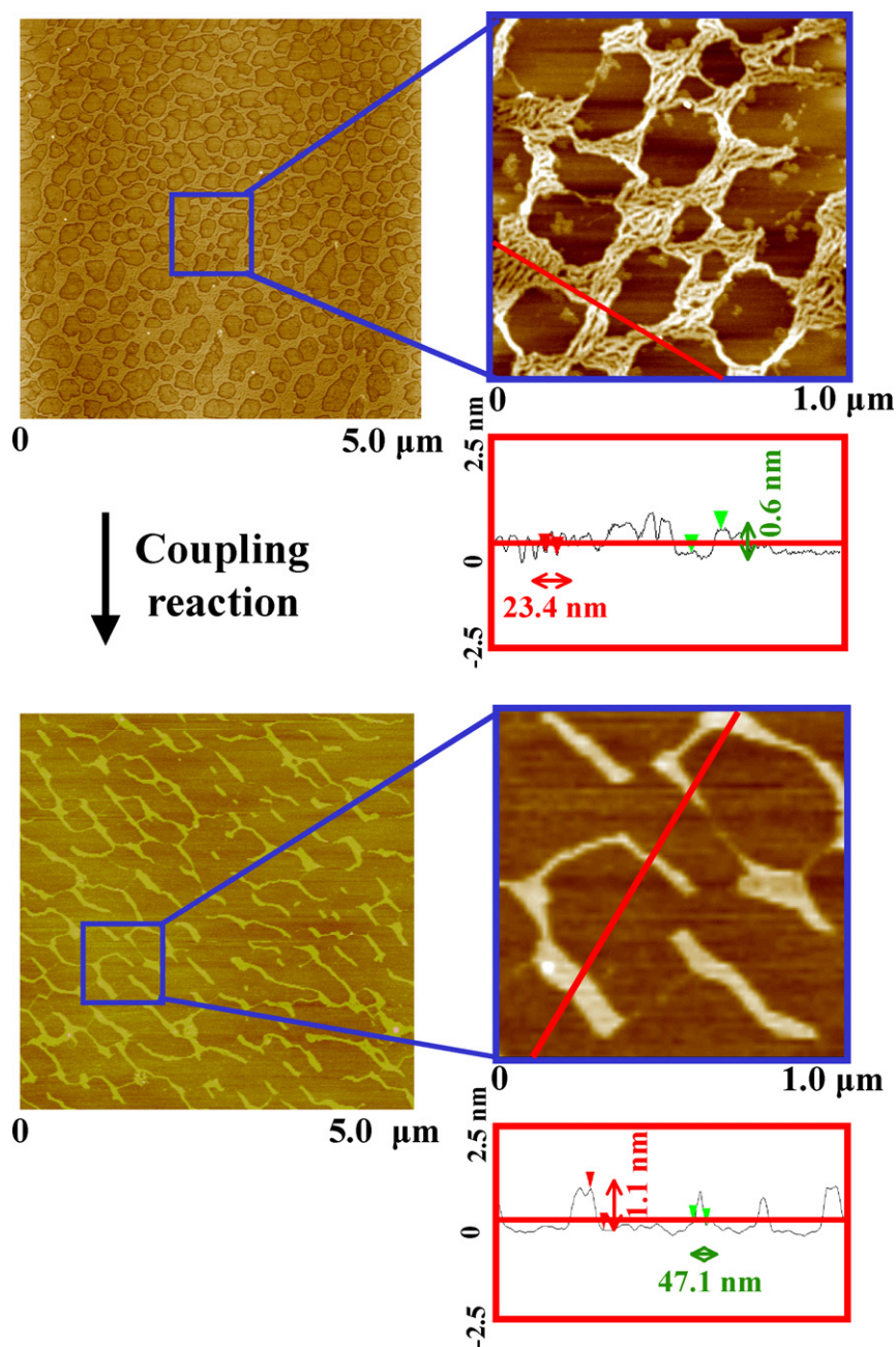
Fig. 3. AFM images and section analyses of NaHA and its coupling-reacted composite with dendrimer at a ratio of [1/0.01]. NaHA concentration = 0.004 wt%.
