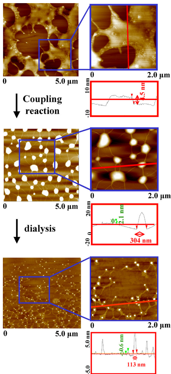
Fig. 4. AFM images and section analyses of NaHA, its coupling-reacted composite with dendrimer at a ratio of [1/0.01], and the dialyzed composite. NaHA concentration = 0.04 wt%.
