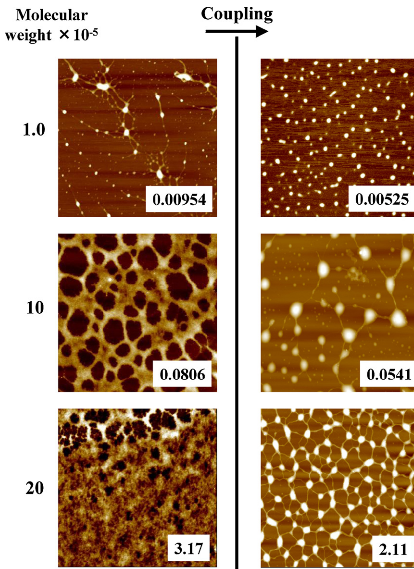
Fig. 7. AFM images of three NaHAs with different molecular weights and their coupling-reacted composites with dendrimer at [1/0.01]. NaHA concentration = 0.04 wt%. Size: 5 \mu\text{m} \times 5 \mu\text{m} . Inset: numerical values of reduced viscosities \eta_{\text{red}} .
