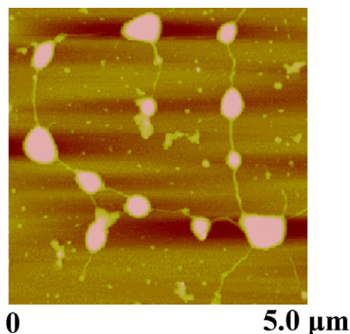
Fig. 5. An AFM image of a noncoupling-reacted composite of HaNA and dendrimer at [1/0.01]. NaHA concentration = 0.04 wt%.
