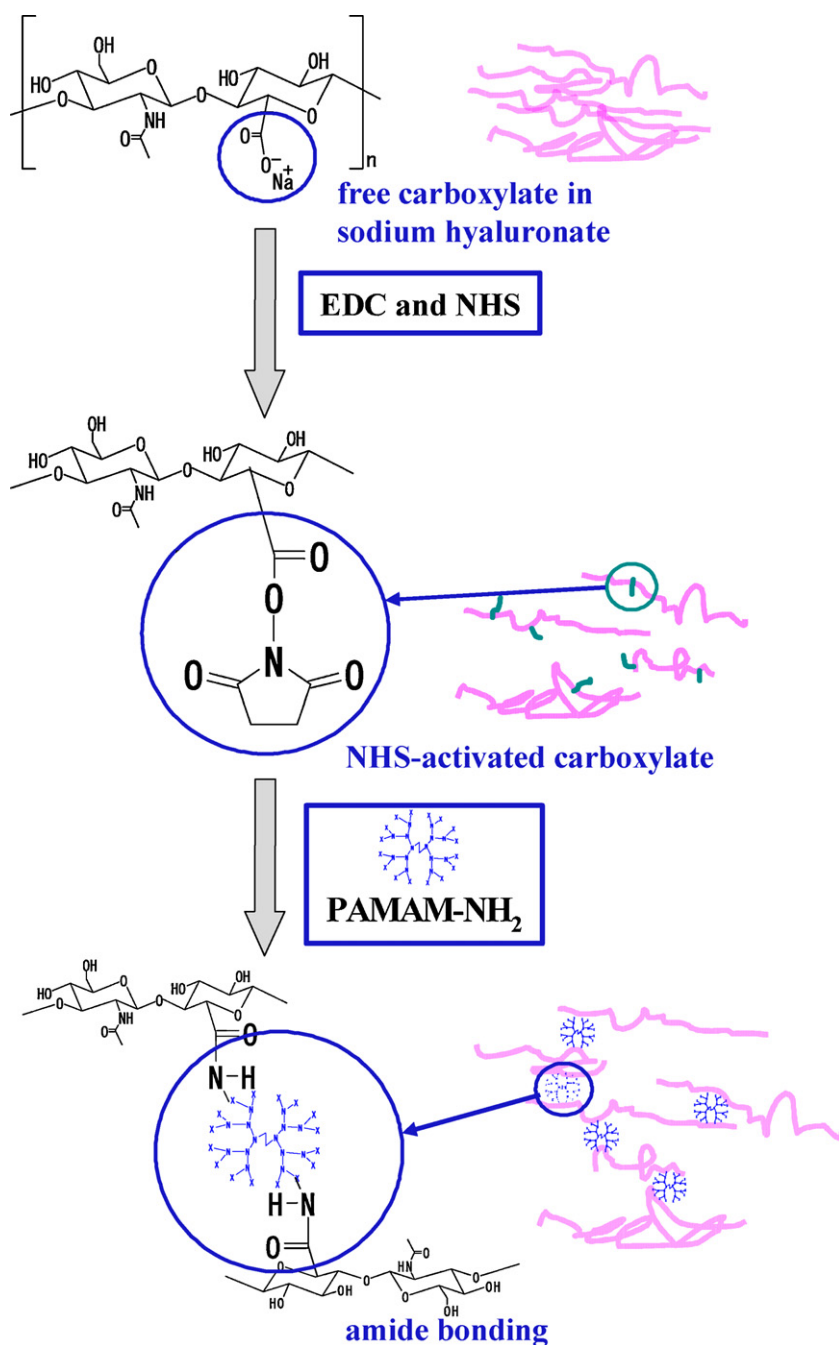
Fig. 1. Schematic illustration of coupling reaction between NaHA and dendrimer.
