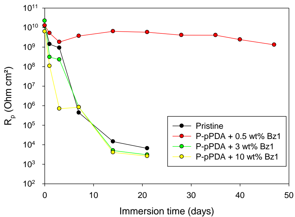
Fig. 13 Evolution over immersion time in 0.1 M NaCl of the calculated pore resistance
