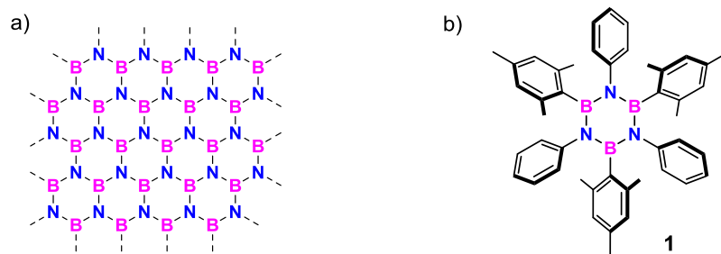
Fig. 1 a) 2D structure of h-BN; b) chemical structure of borazine derivative 1
