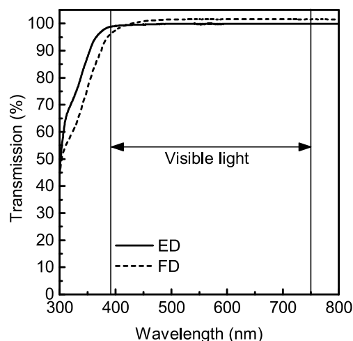
Fig. 4. UV-Vis spectra of ED and FD, showing that both adhesives are transparent in the visible light range.
