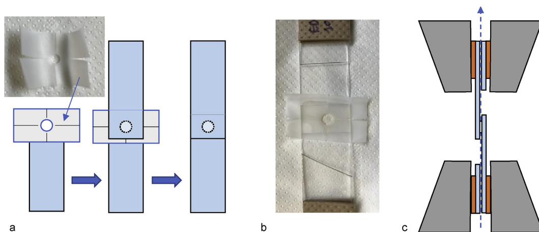
Fig. 2. (a) Scheme of the preparation of the lap-shear specimens and photo of the PTFE mask; (b) photo of a cured specimen before removal of the mask, showing also the glass and rubber spacers; (c) scheme of the lap-shear specimen mounted in the tensile test set-up.
