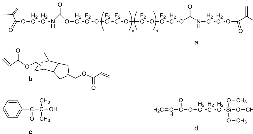
Fig. 1. Chemical structures of (a) Fluorolink ® MD 700 oligomer; (b) Ebecryl ® 130 oligomer; (c) Darocur ® 1173 photoinitiator; (d) 3-(acryloyloxy) propyl-trimethoxysilane coupling agent (silane).
