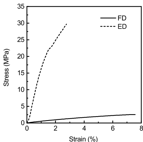
Fig. 5. Representative stress-strain curves for photocured FD and ED resins.
