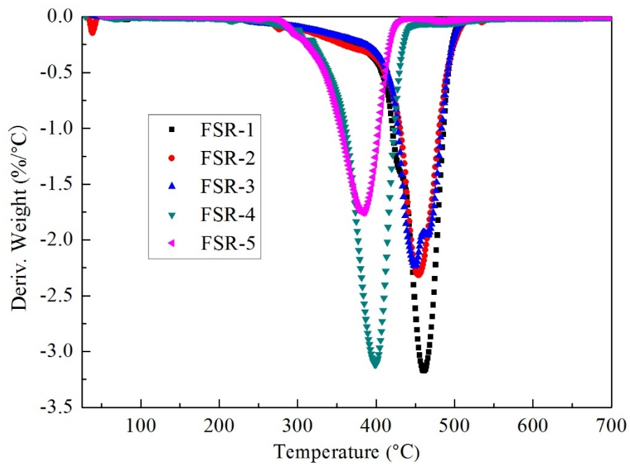
Fig.5. DTG curves of cured FSR
