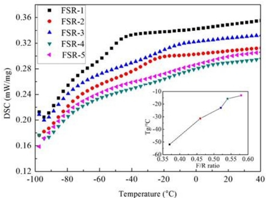
Fig. 6. DSC curve of cured FSR
