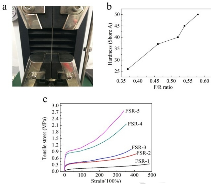
Fig. 7. Mechanical properties of cured FSR. a, Photographs of a cured FSR film during stretching process. b, Hardness of cured FSR with different F/R ratios. c,
