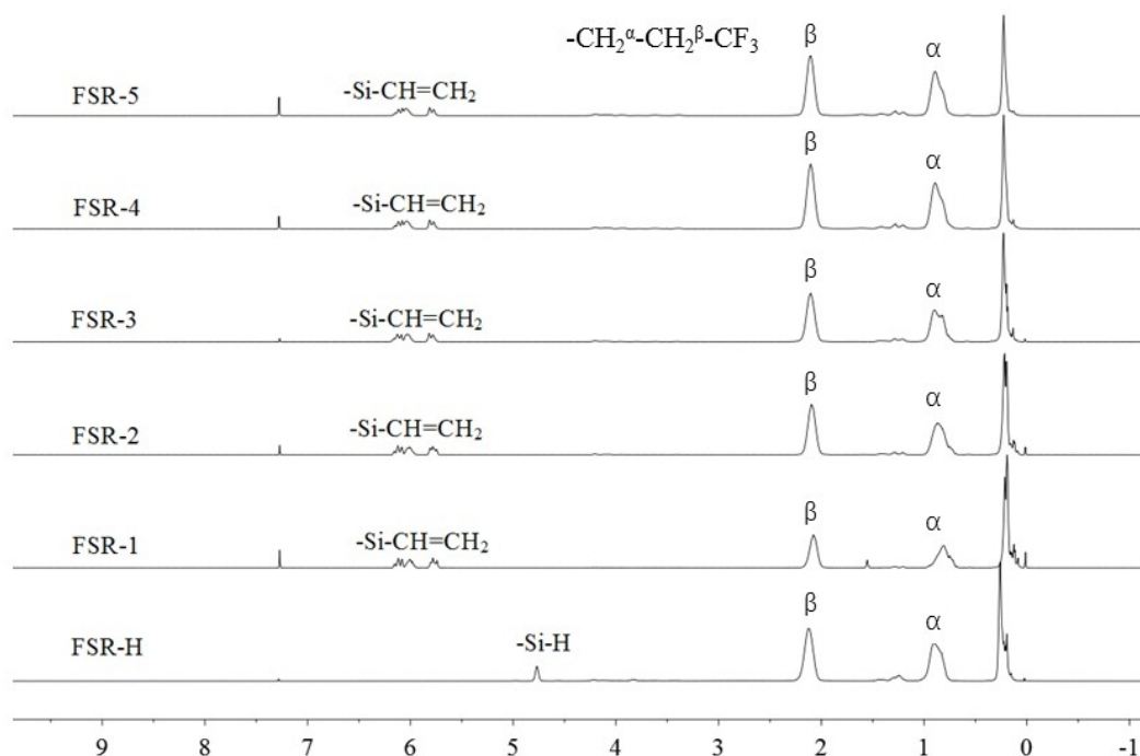
Fig.2. ^1\text{H} NMR of FSR
