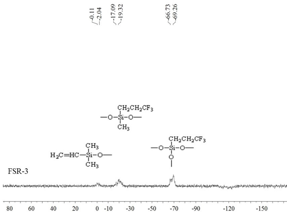
Fig.3. ^{29}\text{Si} NMR of FSR
