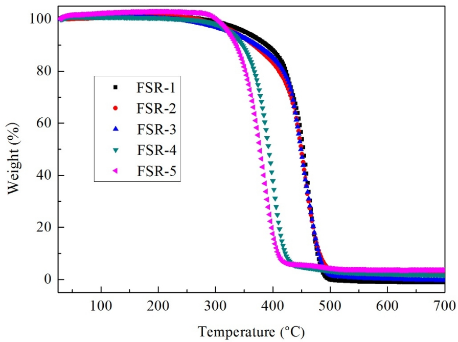
Fig.4. TGA curves of cured FSR
