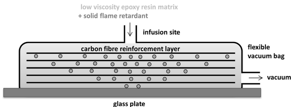
Fig. 6. The suspected “deep filtration” scenario of solid flame retardants during vacuum infusion.
