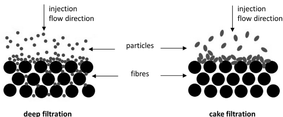
Fig. 1. Illustration of deep filtration and cake filtration mechanisms.
