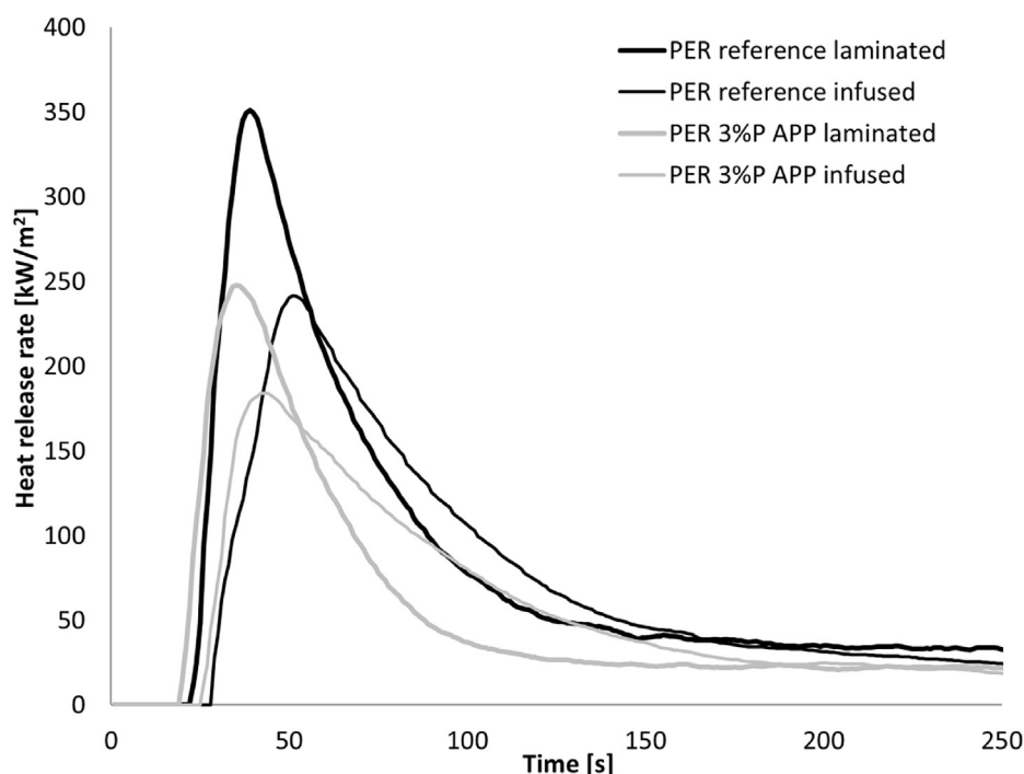
Fig. 5. Heat release rate of carbon fibre reinforced, reference and flame-retarded composites made by hand lamination followed by hot pressing or by vacuum infusion.
