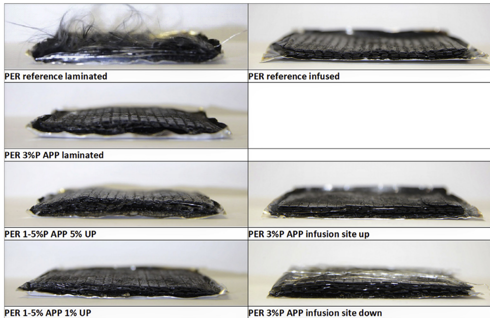
Fig. 9. MLC residues of the reference and flame-retarded carbon fibre reinforced composites made by hand lamination followed by hot pressing or by vacuum infusion.
