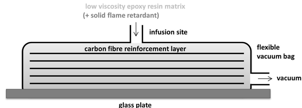
Fig. 3. Composite processing methods.
