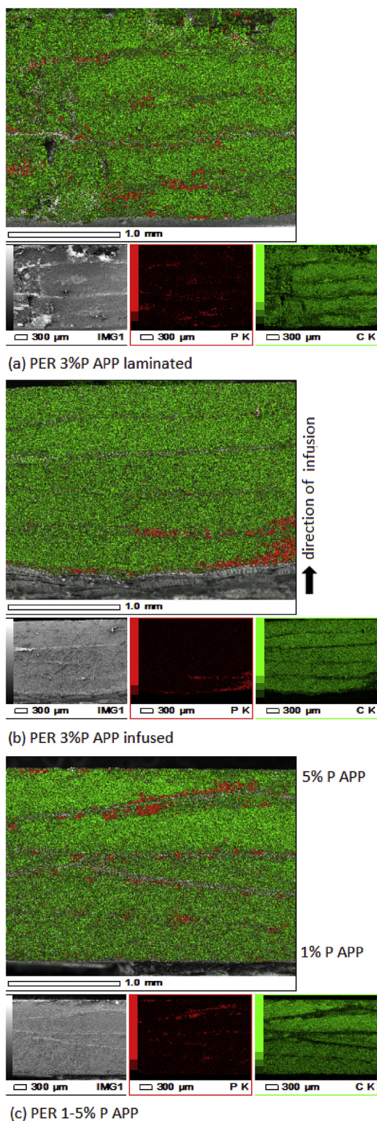
Fig. 11. SEM-EDS map of the cross-section of (a) the PER 3%P APP laminated, (b) the PER 3%P APP infused and (c) the PER 1–5%P APP model composite.
