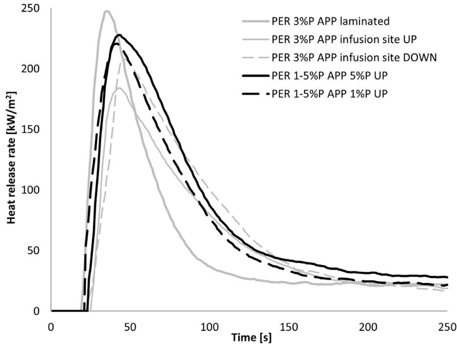
Fig. 8. Heat release rate of flame-retarded carbon fibre reinforced composites made by hand lamination followed by hot pressing or by vacuum infusion.
