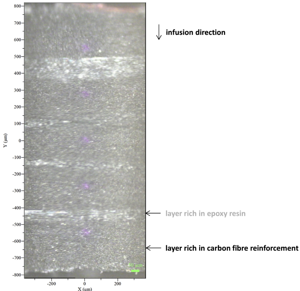
Fig. 10. Optical microscopy image of the cross-section of the PER 3%P APP infused composite.
