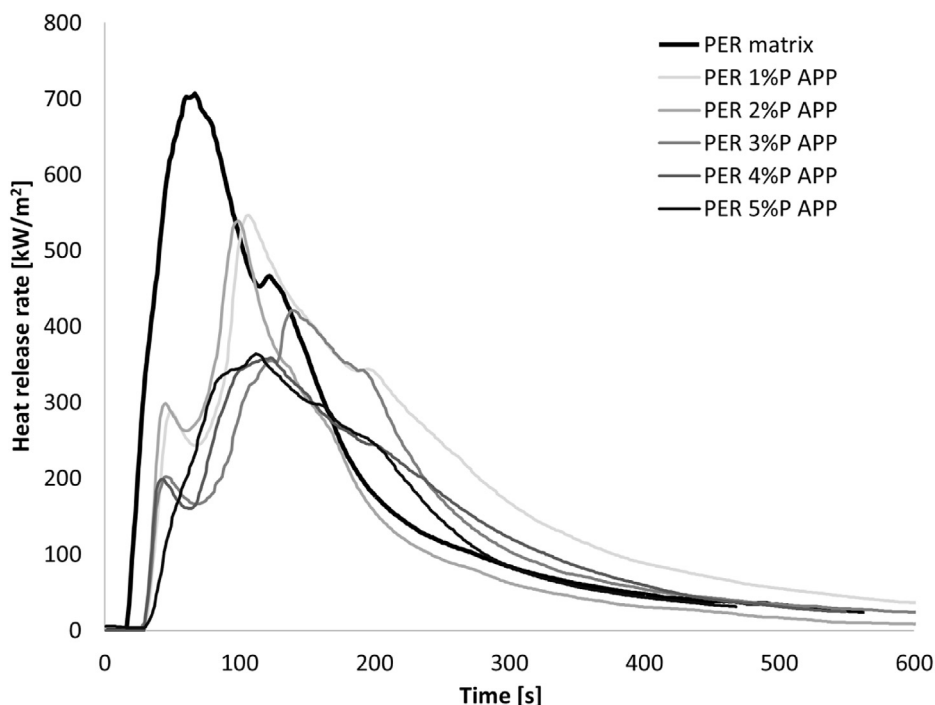
Fig. 4. The effect of gradually increasing APP content on the heat release rate of PER matrix samples.
