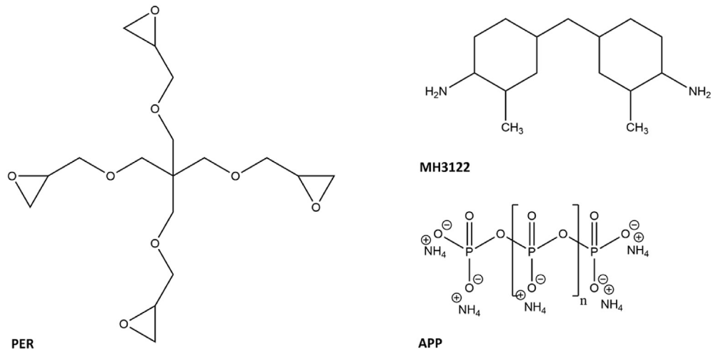
Fig. 2. The chemical structures of the EP monomer (PER), hardener (MH 3122) and FR additive (APP).
