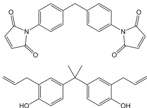
Fig. 5. The structures of 4,4'-bismaleimidodiphenyl methane (top) and diallylbisphenol A (bottom), the most common constituents of BMI systems.
