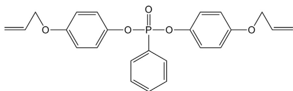
Fig. 16. The chemical structure of a phosphoryl ester containing monomer designed to impart improved flame retardancy.
