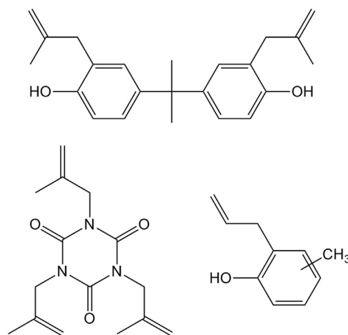
Fig. 18. Chemical structures of potential DABA alternatives: mDABA (left) and TmAIC (middle), and additive allylmethylphenol (right).
