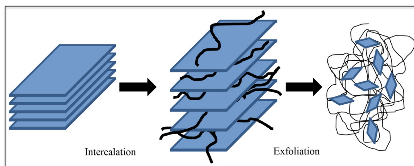
Fig. 29. Schematic of rectorite and the process of exfoliation.
