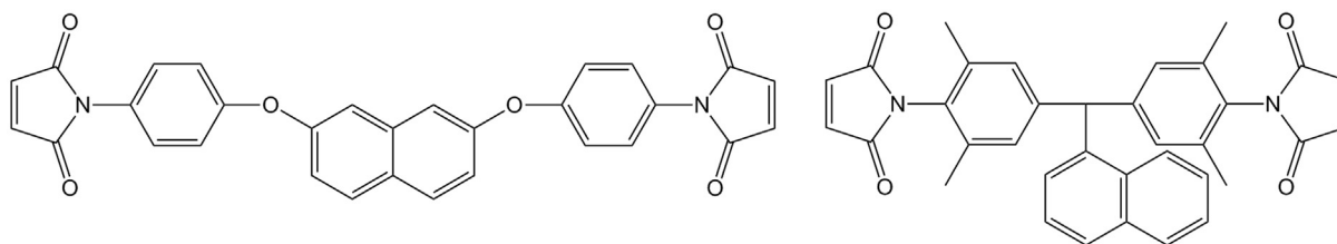
Fig. 13. Examples of BMI monomers that feature naphthalene moieties in their structure.
