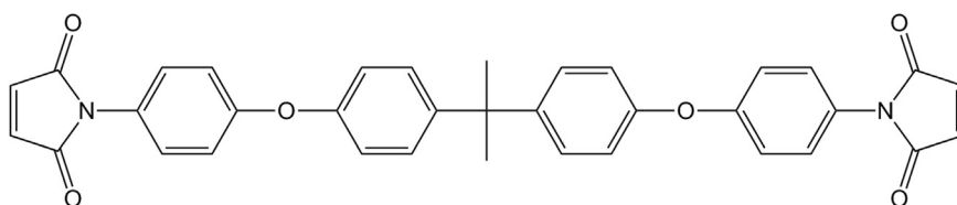
Fig. 9. Structure of 2,2'-bis[4-(4-maleimidophen-oxo)phenyl]propane (BMPP).
