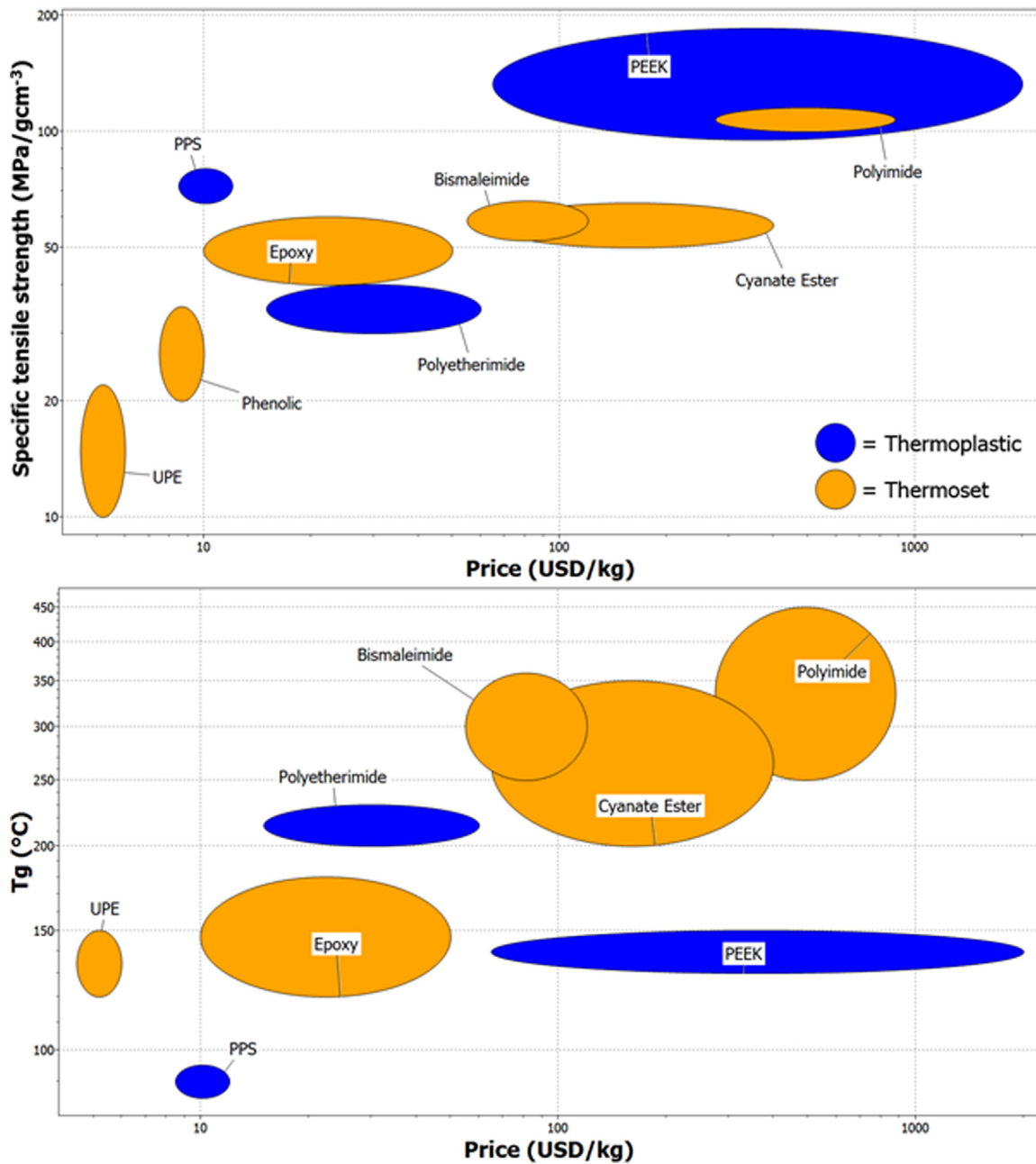
Fig. 2. Comparative properties of advanced resins (redrawn from [3]). Key: UPE = Unsaturated Polyester, PPS = poly(phenylene sulphide), PEEK = poly(ether ketone).
