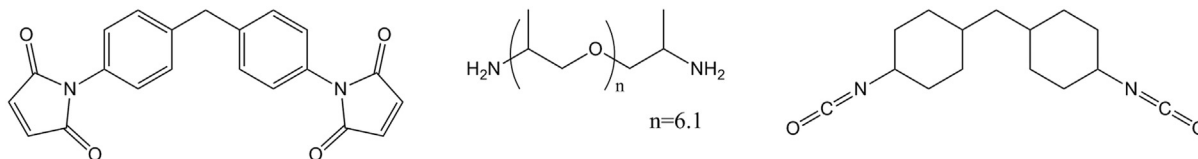
Fig. 30. Components of the BMI based shape memory polymer.
