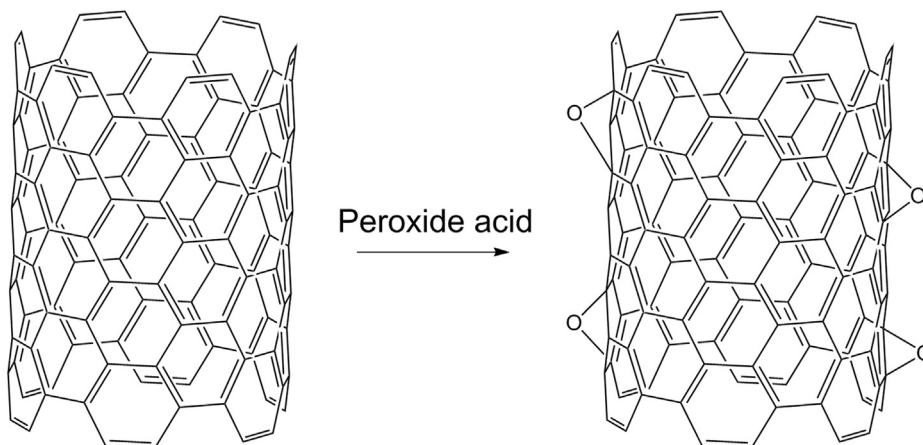
Fig. 26. Surface Functionalisation of carbon nanotubes.
