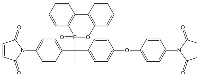
Fig. 15. The chemical structure of a DOPO containing BMI monomer designed to impart improved flame retardancy to the resin.
