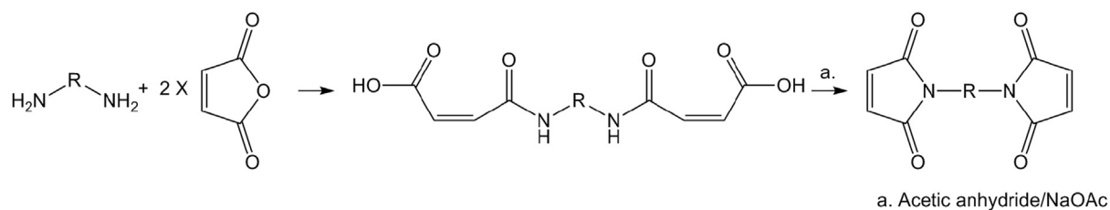
Fig. 3. Typical synthetic mechanism for commercial BMIs.
