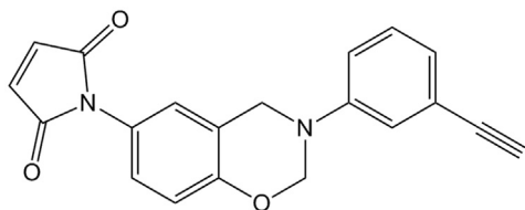
Fig. 25. Monomer containing three different thermosetting functionalities.
