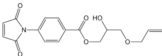
Fig. 10. Structure of 3-(allyloxy)-2-hydroxypropyl 4-maleimidobenzoate.
