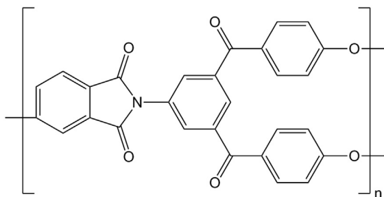
Fig. 20. Chemical structure of the hyperbranched poly(ether-ketone-imide) modifier.
