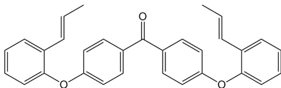
Fig. 8. Structure of reactive modifier Compimide TM123.
