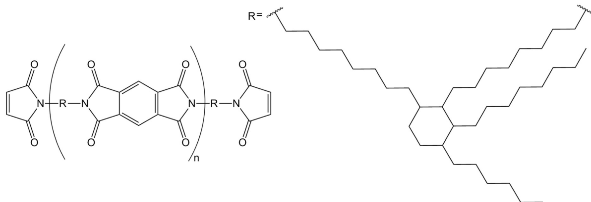
Fig. 17. The structure of a C 36 containing BMI monomer ( n \approx 3 ).
