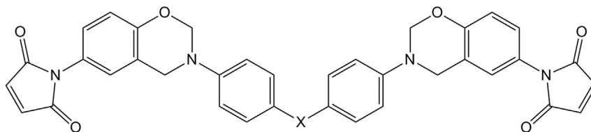
Fig. 24. Monomer containing both BZ and BMI functionalities.
