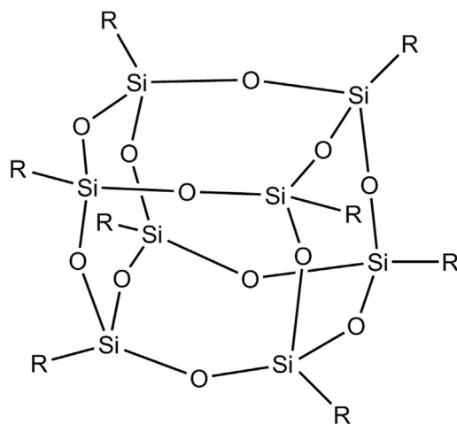
Fig. 28. The general structure of the most common form of POSS reagent, where R is commonly a branched alkyl chain e.g. isooctyl or isobutyl with one or more R groups replaced with a reactive functional group).
