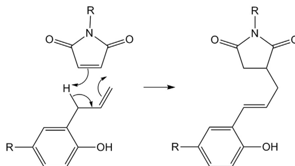
Fig. 6. Hypothesised mechanism of the ene reaction that is thought to occur between allyl and maleimide groups (N.B., half of each molecule shown).
