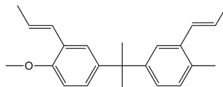
Fig. 19. Propenyl containing building block that can be incorporated into poly(aryl ether) and its derivatives.
