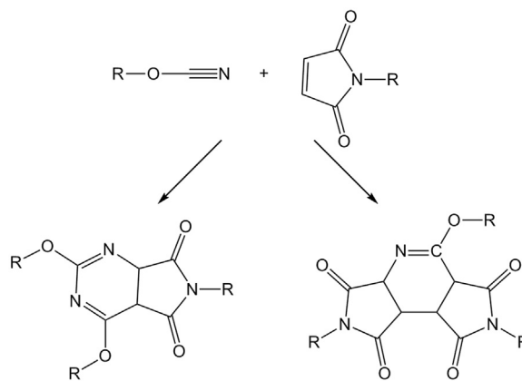
Fig. 22. Reaction schemes which have been proposed for the co-reaction between BMI and CE monomers.
