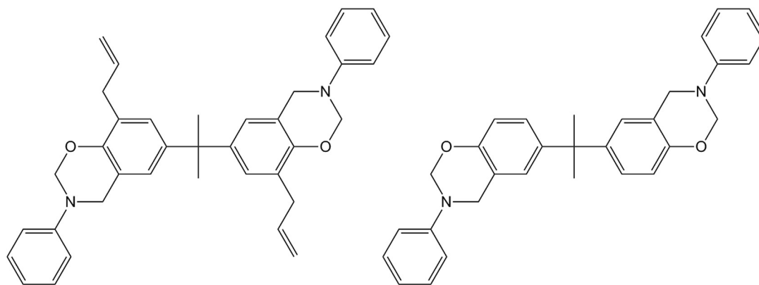
Fig. 23. Examples of benzoxazine monomers diallyl BA-a (left) and BA-b (right) that have been used to modify BMIs.
