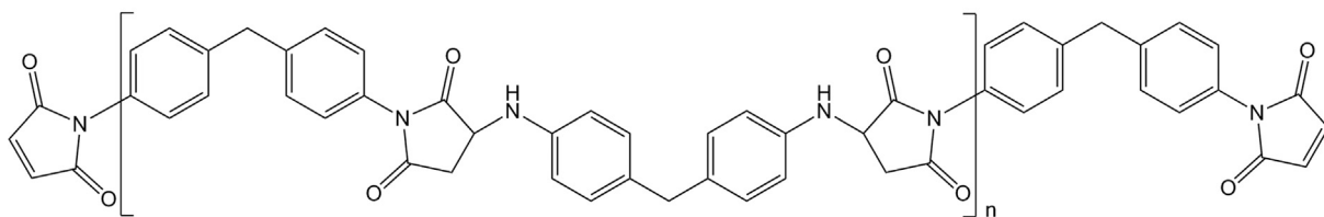
Fig. 4. Structure of commercial BMI (Kerimid 601 and Compimide 200).
