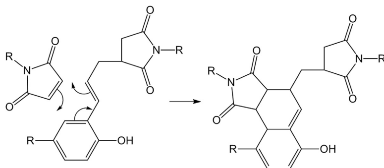
Fig. 7. Hypothesised mechanism of the Diels-Alder reaction originally thought to succeed the ene reaction (N.B., half of each molecule shown).
