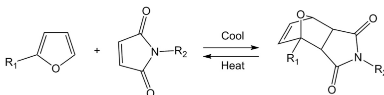
Fig. 31. The reversible Diels-Alder reaction between furan and maleimide.
