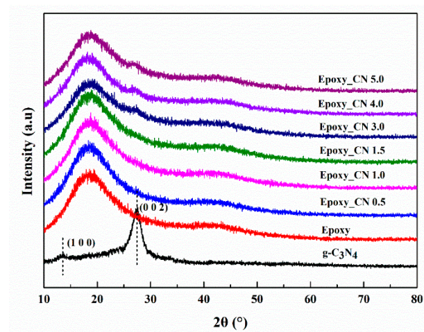
Figure 5. X-ray Diffraction (XRD) patterns of the epoxy and g-C 3 N 4 /epoxy nanocomposites.
