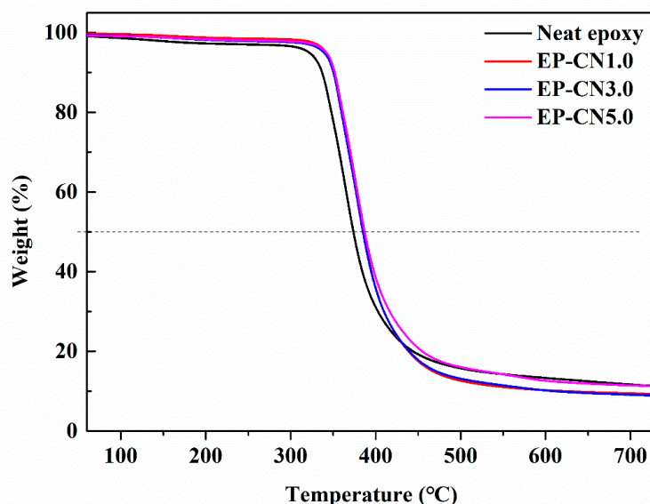
Figure 14. Gravimetric thermograms (TG) of the epoxy and g\text{-C}_3\text{N}_4 /epoxy nanocomposites.
