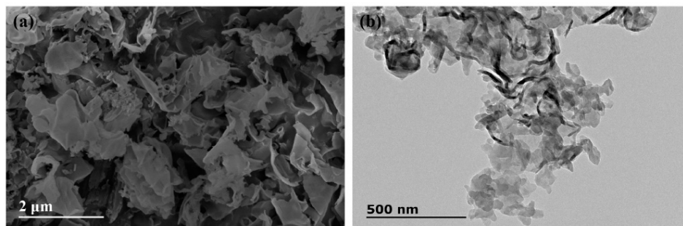
Figure 3. Micrograph of g-C 3 N 4 : (a) scanning electron microscope (SEM); (b) transmission electron microscopy (TEM).
