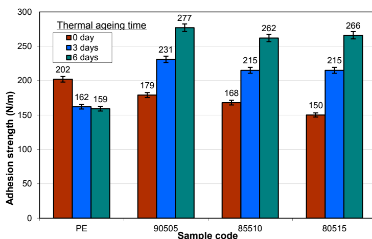
Figure 8. Adhesion strength of PE/amino-POSS/FeSt 3 blends to paperboard.
